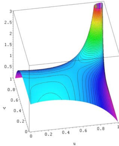
plot of c(u, v)
