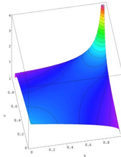
plot of c(u, v)
