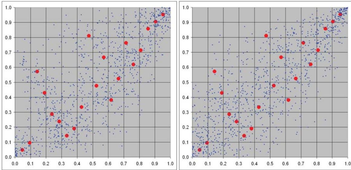
Bernstein copula fit
