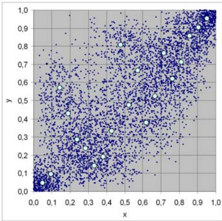
Figure 7: Bernstein copula
