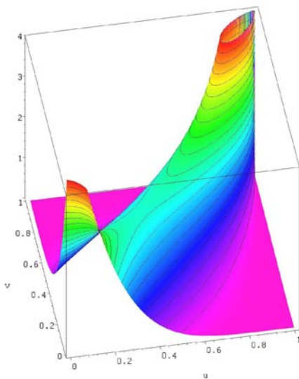
Figure 1: Density of a bivariate negative binomial copula, a = 5
