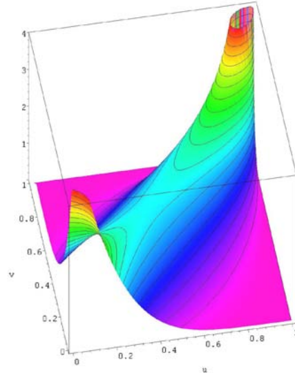
Figure 2: Density of a bivariate Poisson copula, a = 5
