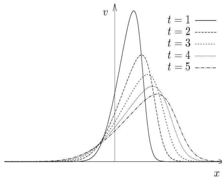
Figure 1: Sketch of self-similar decay of the amplitude in a comoving frame in (1.6).
