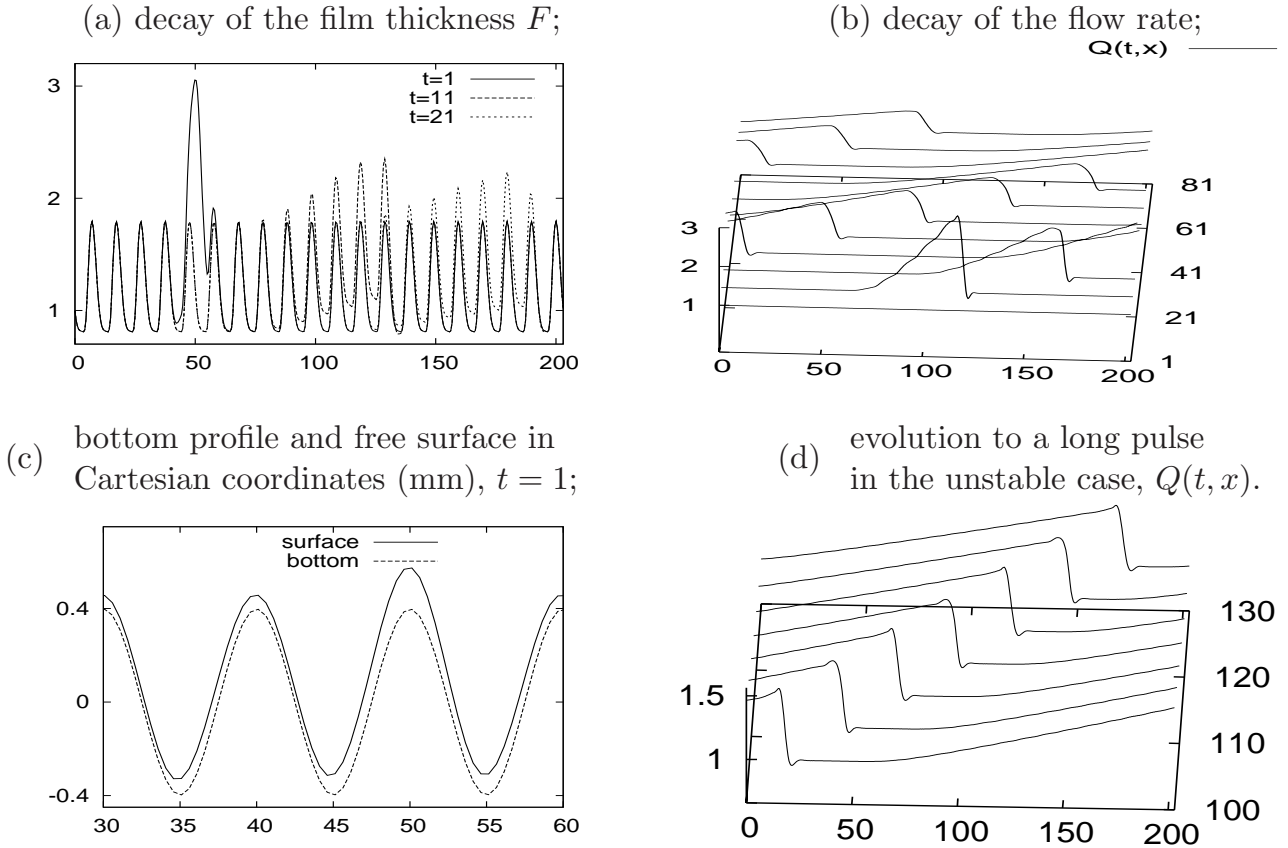
Figure 2: Numerical simulations of (1.1), (1.2) in the stable case (a)-(c) and the unstable case (d), with periodic boundary conditions. In (a)-(c) we used a sinusoidal bottom with amplitude a = 0.4\text{mm} and wavelength \lambda=10\text{mm} (bottom profile \hat{b}(\hat{x}) = a \cos(\frac{2\pi}{\lambda}\hat{x}) ). The mean film thickness is h \approx 0.06\text{mm} , inclination angle \alpha = 60^\circ , and the fluid parameters correspond to water, which yields \delta \approx 0.037 , \zeta = 0.25 , B_i \approx 3.25 and R = 0.6 . The initial condition is F = f_s + 2/\cosh((x - 50)/5) , Q = q_s \equiv 1 . Although R is larger than the critical Reynolds number over flat bottom, which is R_{\text{crit}} \approx 0.48 , the stationary solution is stable and the perturbation decays in the self-similar way predicted by (1.6). (a) shows F at times as indicated, while (b) shows the evolution of Q . In the latter we directly see the envelope t^{-1/2} f_{z_0}(t^{-1/2}(x + c_1 t)) since \Phi_2^1(0, \cdot) \equiv 1 , while \Phi_1^1(0, x) = \frac{df_s}{dq_s}(x) is \gamma -periodic. To illustrate the physical situation, panel (c) shows the bottom contour and the free surface at initial time t = 1 in dimensional (mm) cartesian coordinates, between the 4 th and 6 th bottom wave. Finally, panel (d) shows Q (for large time) after we increased \alpha to 90^\circ . Here (f_s, q_s)^\top has become unstable: the perturbation does not decay to 0, but instead evolves into a long pulse. We expect that this situation can be described by a generalized KS equation, see, e.g., [CD02, PSU07] for the situation over flat bottoms, and [UW07] for a model problem for wavy bottoms.
