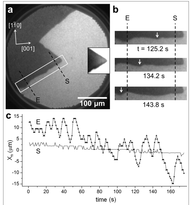
FIG. 1: Experimental observation of interface excitations in the \text{NH}_3 + \text{O}_2 reaction on Rh(110). Experimental conditions: T=740\text{ K} , p(\text{NH}_3)=3.85 \times 10^{-5}\text{ mbar} , p(\text{O}_2)=1.35 \times 10^{-5}\text{ mbar} . (a) PEEM image showing the interface between oxygen-rich (dark) and nitrogen-rich surface area (bright). The inset representing an enlarged view of the interface region near S shows the formation of dark boundary layer at the interface within the oxygen phase. (b) Enlarged view of the region marked in (a) showing the pulse-like propagation of an interface modulation. (c) Position vs. time plots showing the temporal variation of the interface position. The data were taken from cross sections normal to the line E-S in (a) with the coordinate x_n in (c) corresponding to direction north-west in (a). See also the movie in the supplemental material †.
