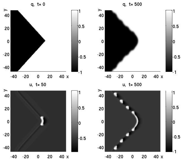
FIG. 4: Numerical integration of (1) in frame moving with speed \eta = 3c_1/4 = -0.15 . Parameters d_u = 0.09, d_v = 0.01, d_{uq} = 0.1, \beta = 0.2, \delta = 0.5, \varepsilon = 0.03, \gamma = -0.05, a = -0.1 . IC for q is the wedge (4) with x_0 = L/4, m = 1 , ICs for (u, v) are (u_s, v_s) . BC according to (6) with \xi_0 = -3L/4 .
