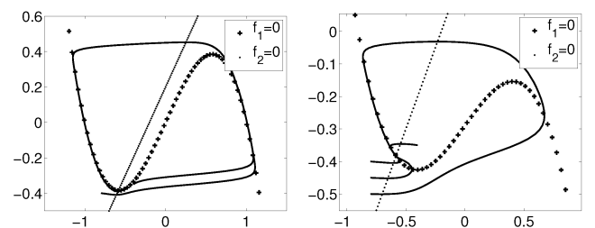
FIG. 3: Influence of q on the u, v system (1a,b), which for q^2 = 0 (left) is more excitable than for q^2 = 1 (right). Other parameters: \beta = 0.2 , \varepsilon = 0.03 , \delta = 0.5 .
