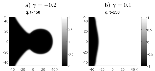
FIG. 5: Same parameters and IC as in Fig.4 except for \gamma .
