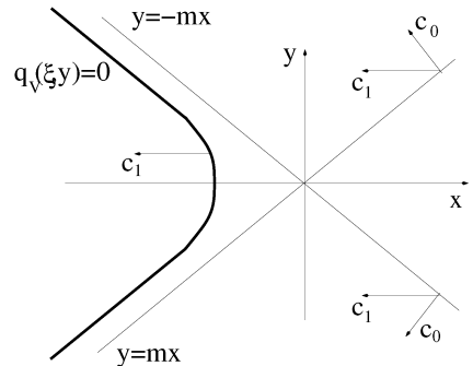
FIG. 2: Heuristics for V-shaped fronts of (3).
